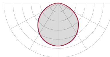
Photometric curve
